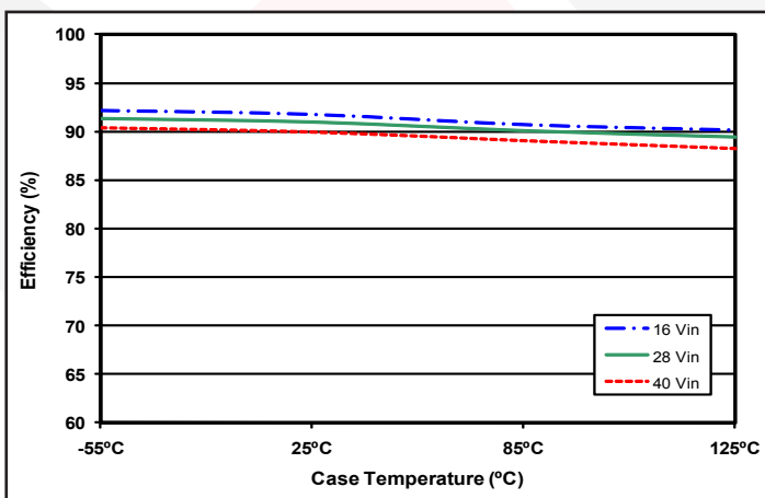
Figure 5: Efficiency at 60% load (3A load on +12V and 3A load on -12V) versus case temperature for Vin = 16V, 28V, and 40V.
