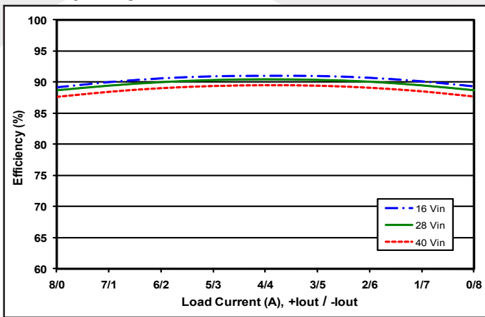
Figure 1: Efficiency vs. output power, from 0 load to full load with 50% load on the +12V output and 50% load on the -12V output at minimum, nominal, and maximum input voltage at 25°C.
