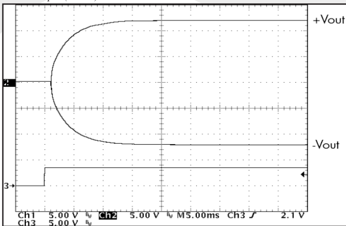
Figure 13: Turn-on transient at full rated load current (resistive load) (5 ms/div). Input voltage pre-applied. Ch 1: +Vout (5V/div); Ch 2: -Vout (5V/div); Ch 3: Enable1 input (5V/div).
