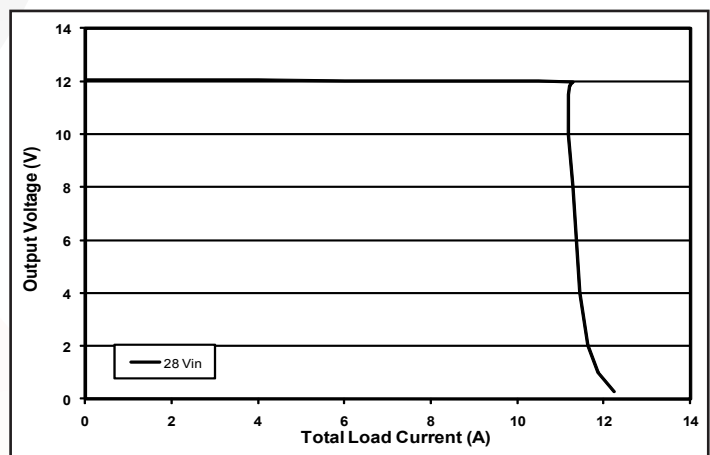
Figure 12: Positive output voltage vs. total load current evenly split showing typical current limit curves.
