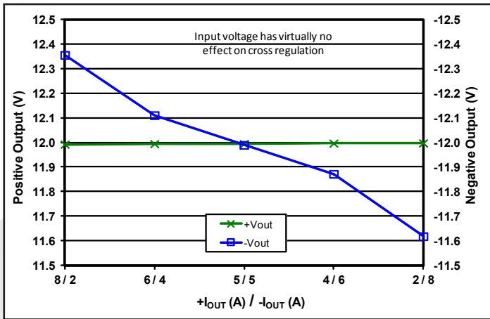
Figure 7: Load regulation vs. load current with power fixed at full load (120W) and load currents split as shown between the +12V and -12V outputs, at nominal input voltage and TCASE = 25°C.
