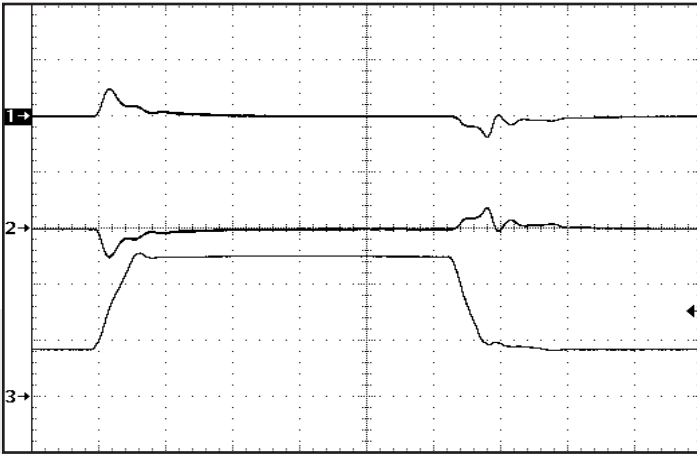
Figure 19: Output voltage response to step-change in input voltage (16V - 50V - 16V). Load cap: 10µF, 100 mΩ ESR tantalum cap and 1µF ceramic cap. Ch 1: +Vout (500mV/div); Ch 2: -Vout (500mV/div); Ch 3: Vin (20V/div).
