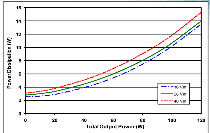
Figure 2: Power dissipation vs. output power, from 0 load to full load with 50% load on the +12V output and 50% load on the -12V output at minimum, nominal, and maximum input voltage at 25°C.
