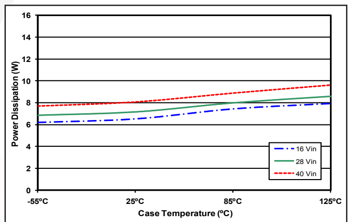
Figure 6: Power dissipation at 60% load (3A load on +12V and 3A load on -12V) versus case temperature for Vin = 16V, 28V, and 40V.
