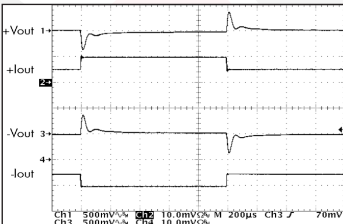
Figure 17: Output voltage response to step-change in total load current (50%-100%-50%) of total Iout (max) split 50%/50%. Load cap: 1μF ceramic cap and 10μF, 100 mΩ ESR tantalum cap. Ch 1: +Vout (500 mV/div); Ch 2: +Iout (5A/div); Ch 3: -Vout (500 mV/div); Ch 4: -Iout (5A/div).
